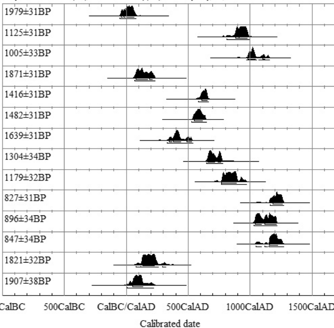
Atmospheric data from Reimer et al (2004), OnCal v3.10, Brook Runway (2005), sub #5 sd.12 prob usg[thms]
