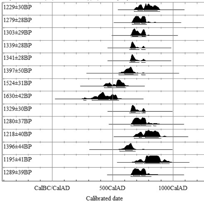
Atmospheric data from Reimer et al (2004),OxCal v3.10 Bronk Ramsey (2005), sub r5 sd.12 prob usg[shom]
